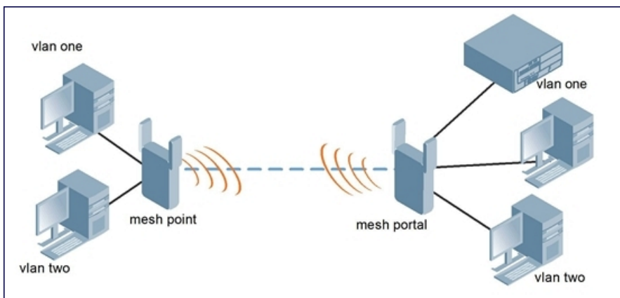
Figure 83 Sample Point-to-Point Deployment
