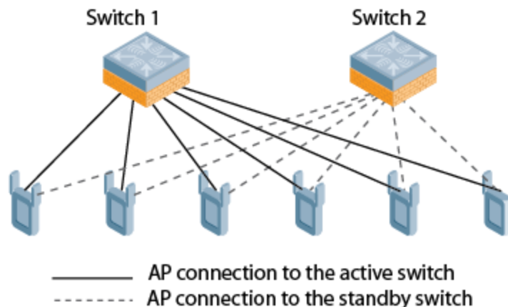
Figure 87 1:1 Active/Standby Deployment
