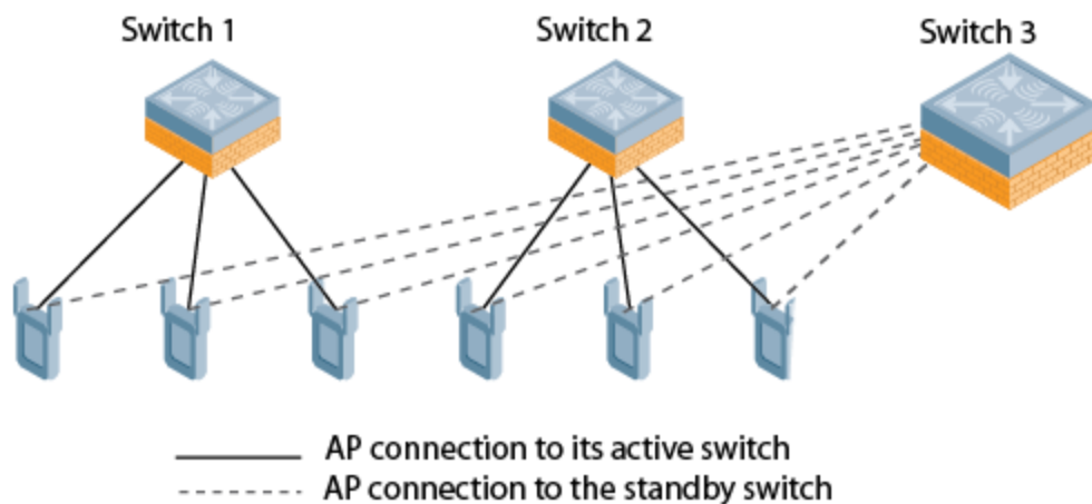
Figure 88 1:1 Active/Standby Deployment
