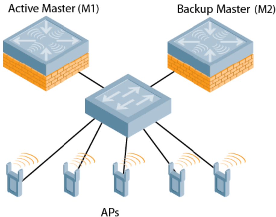
Figure 89 Redundancy with an Active-Backup Master Switch Pair
