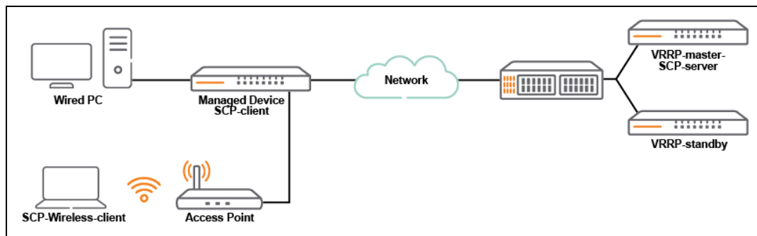
Figure 112 Sample Topology - VRRP Master as SCP Server
