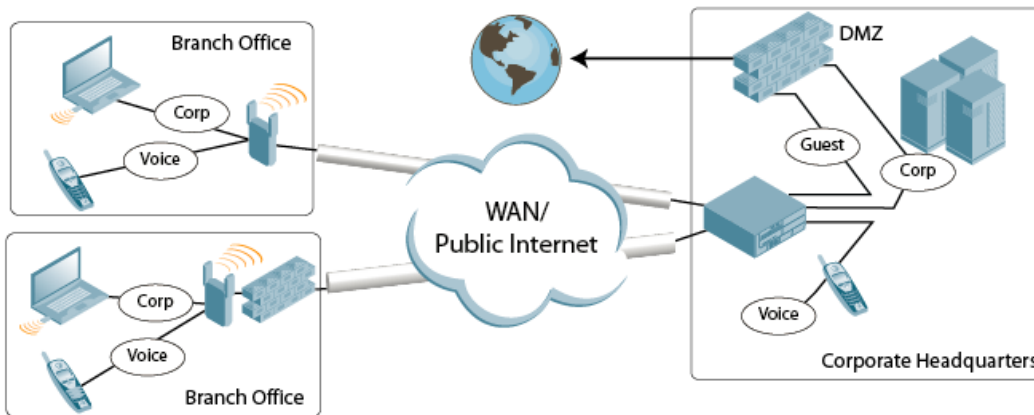
Figure 94 Remote AP with Single Managed device
