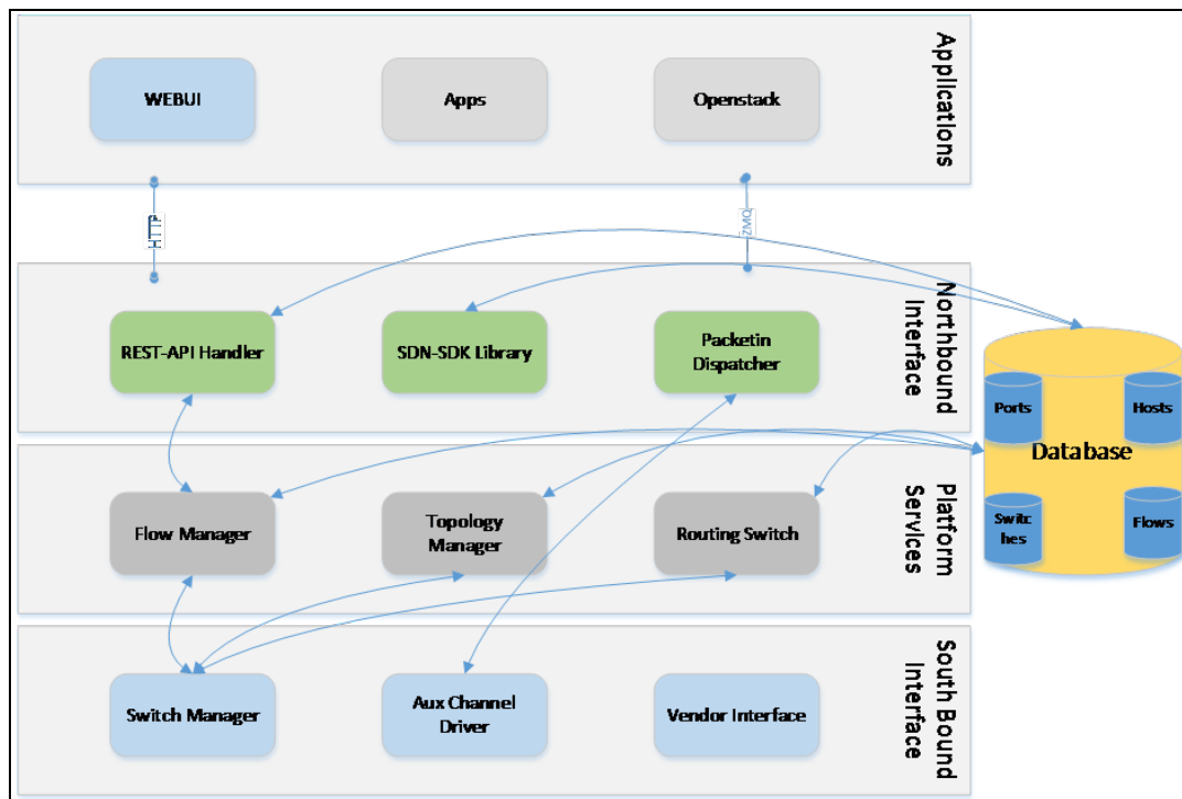
Figure 113 SDN Switch Architecture
